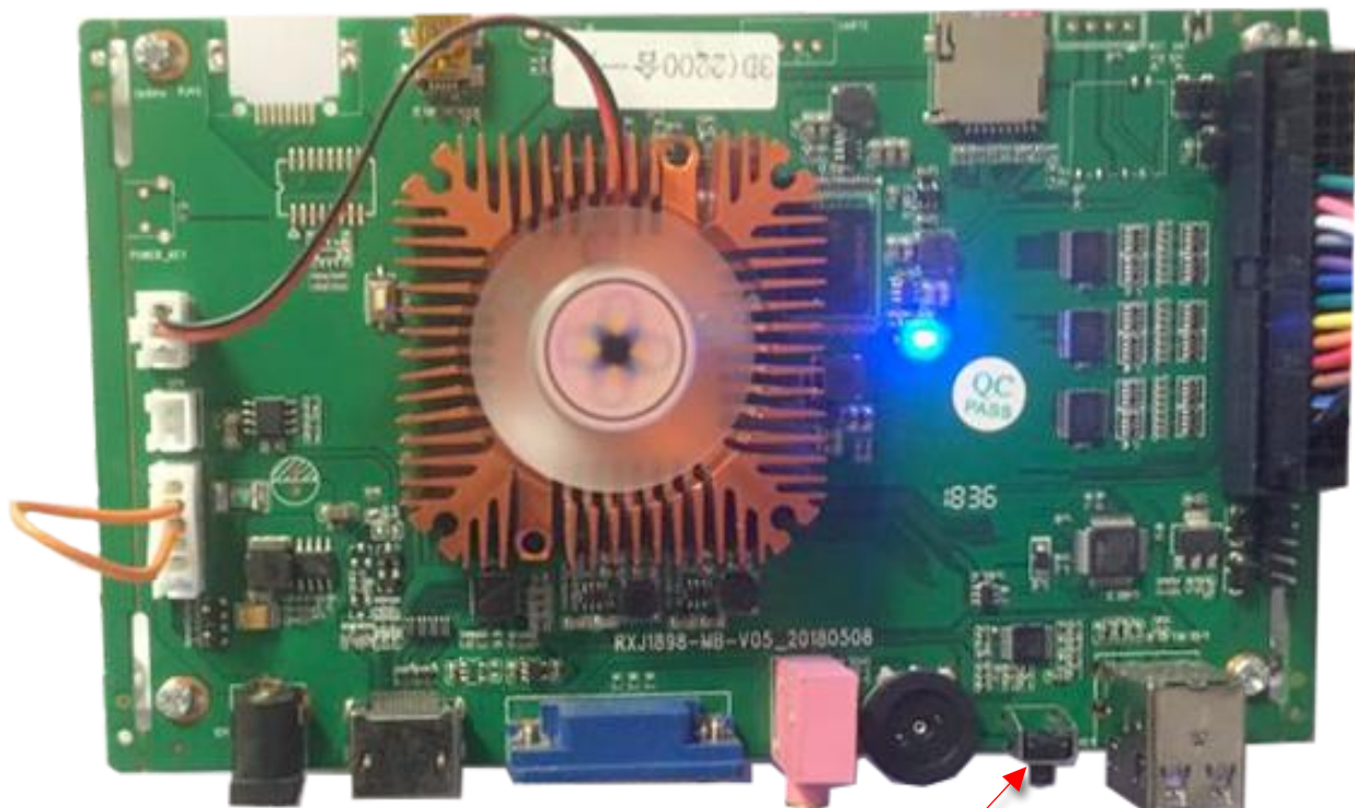
Settings Switch
